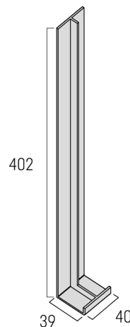
Verbinder 6R38
